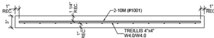
COUPE B-B 1 1/2" = 1'-0"
